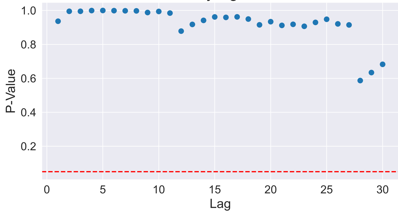
P-value from Ljung-Box test - O3
